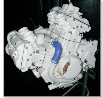
The Desmosedici's engine was prototyped almost entirely from polycarbonate using the FDM process.
